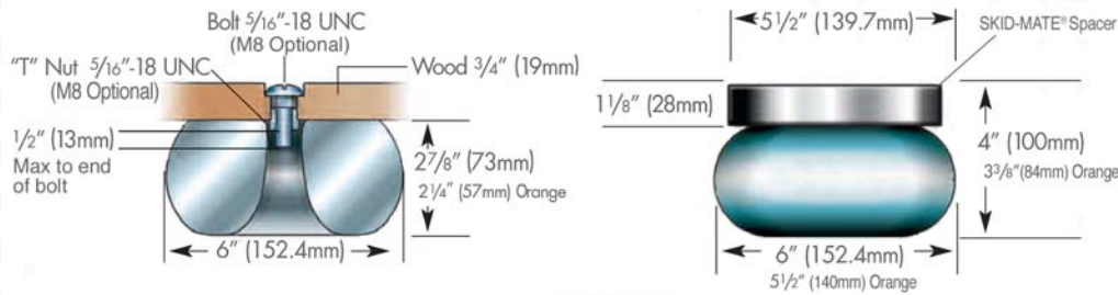
Typical SKID-MATE® pallet for heavy and sensitive loads.
